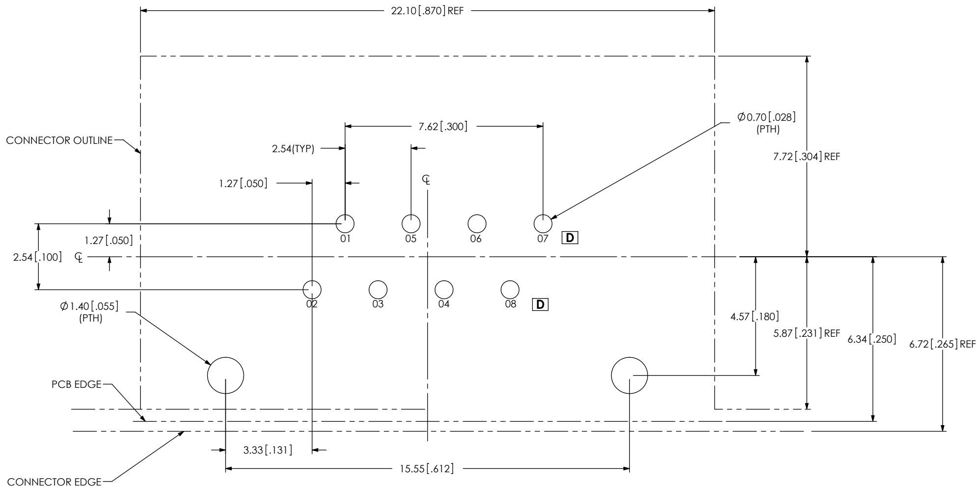
FIG 1 RPBE-01-01-E SHOWN ALL DIMENSIONS ARE SYMMETRIC ABOUT THE CENTERLINE
