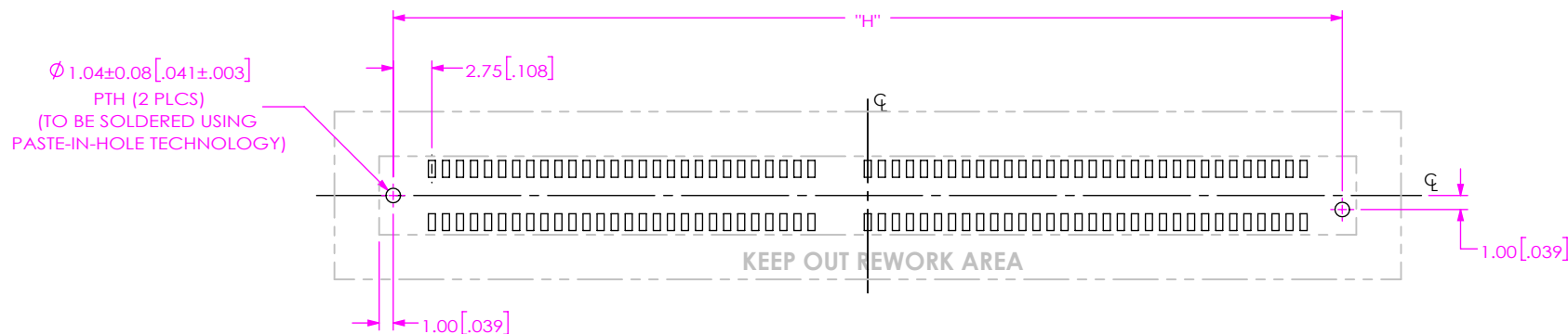
FIG 4 HSEC1-060-01-X-DV-WT FOOTPRINT SHOWN (DIFFERENT AS SHOWN, OTHERWISE SAME AS FIG 2) USE FOR -040, -050, -060, -070, *-080, *-090 & *-100 POSITIONS WITH -WT OPTION (* = NOT TOOLED)
