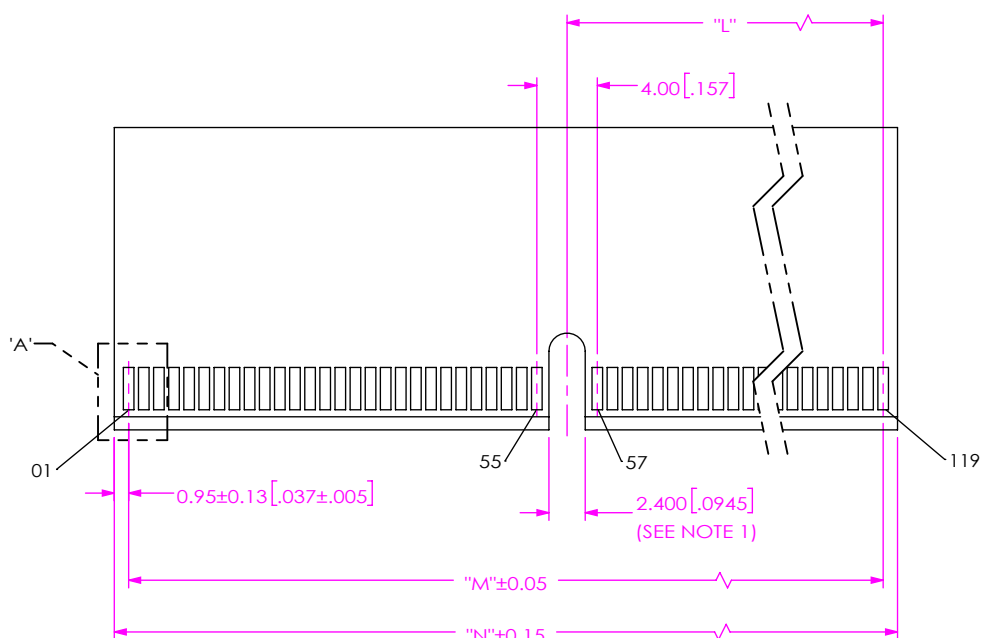
FIG 7 HSEC1-060-01-X-DV-X-XX MATING CARD SHOWN
