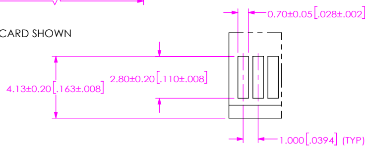
DETAIL 'A' SCALE 4:1
