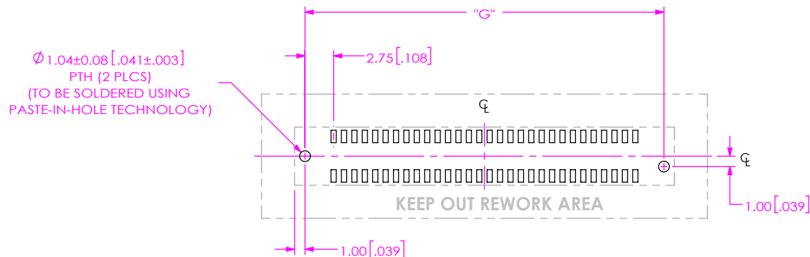
FIG 3 HSEC1-030-01-X-DV-WT FOOTPRINT SHOWN (DIFFERENT AS SHOWN, OTHERWISE SAME AS FIG 1) USE FOR -010, -020 OR -030 POSITIONS WITH -WT OPTION
