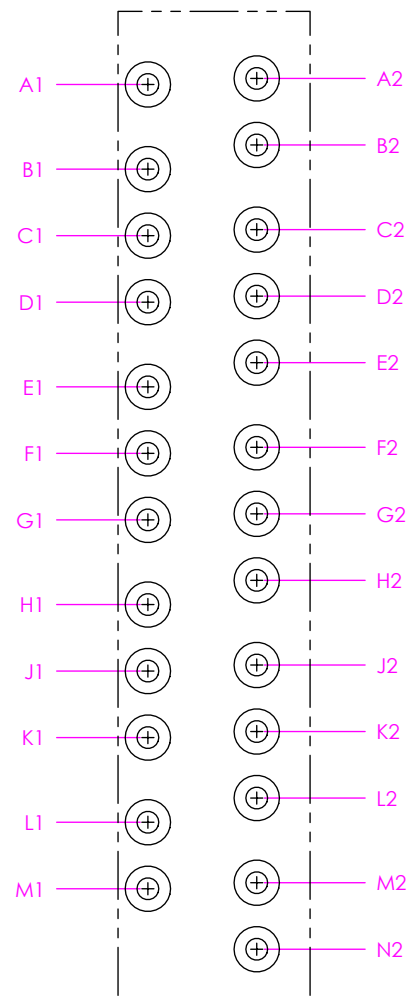
DETAIL 'A' SCALE 10 : 1 (-LC PINOUT)
