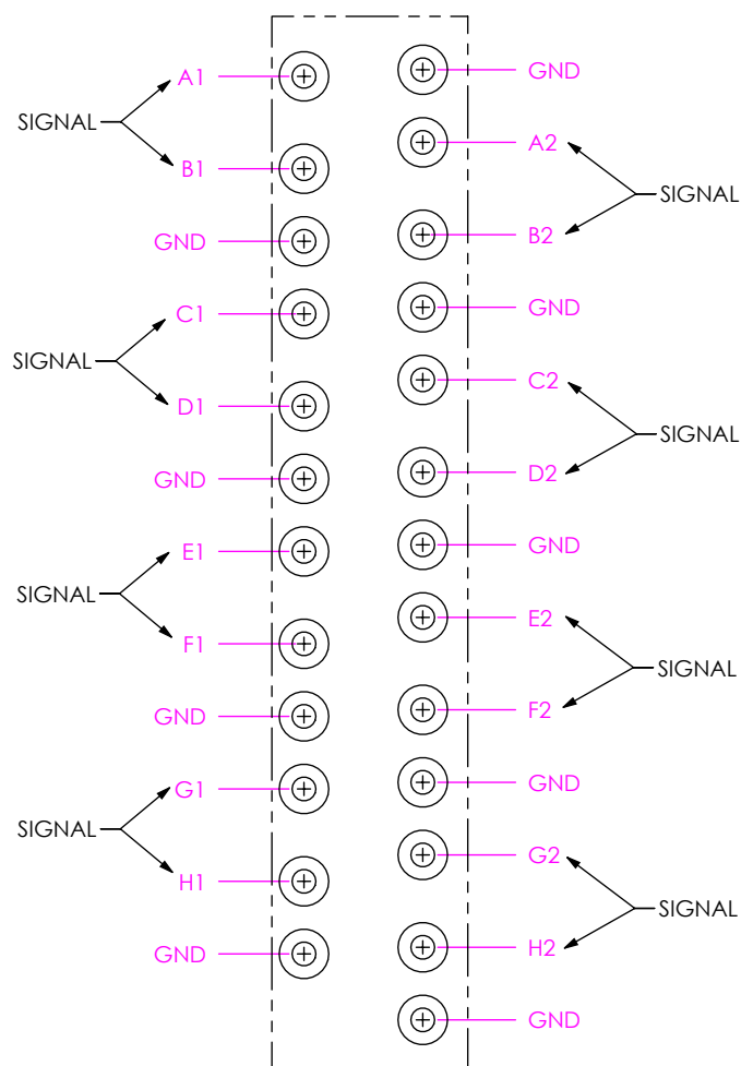
DETAIL 'A' SCALE 8 : 1 (-HS PINOUT)
