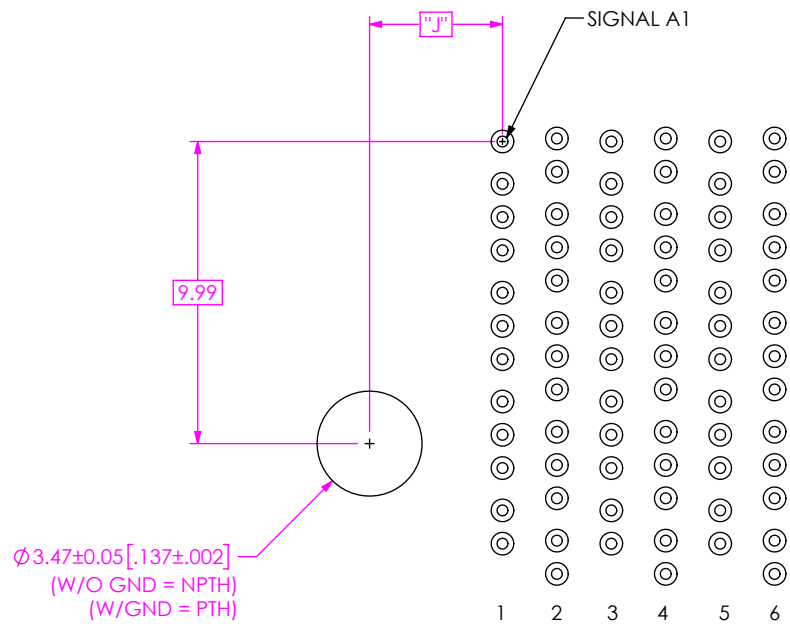
FIG 6 (STAND ALONE, LEFT PCB MOUNTED GUIDE PIN) (SAME AS FIG 1, EXCEPT AS SHOWN)
