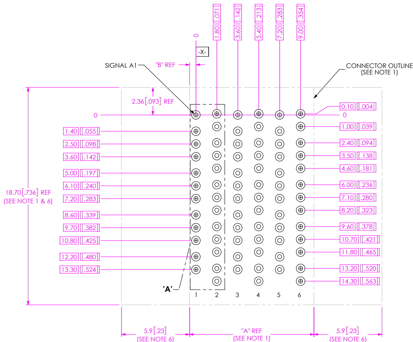
FIG 1 (HDTM-4-06-X-X-VT-X-X FOOTPRINT SHOWN)
