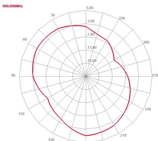
E plane
