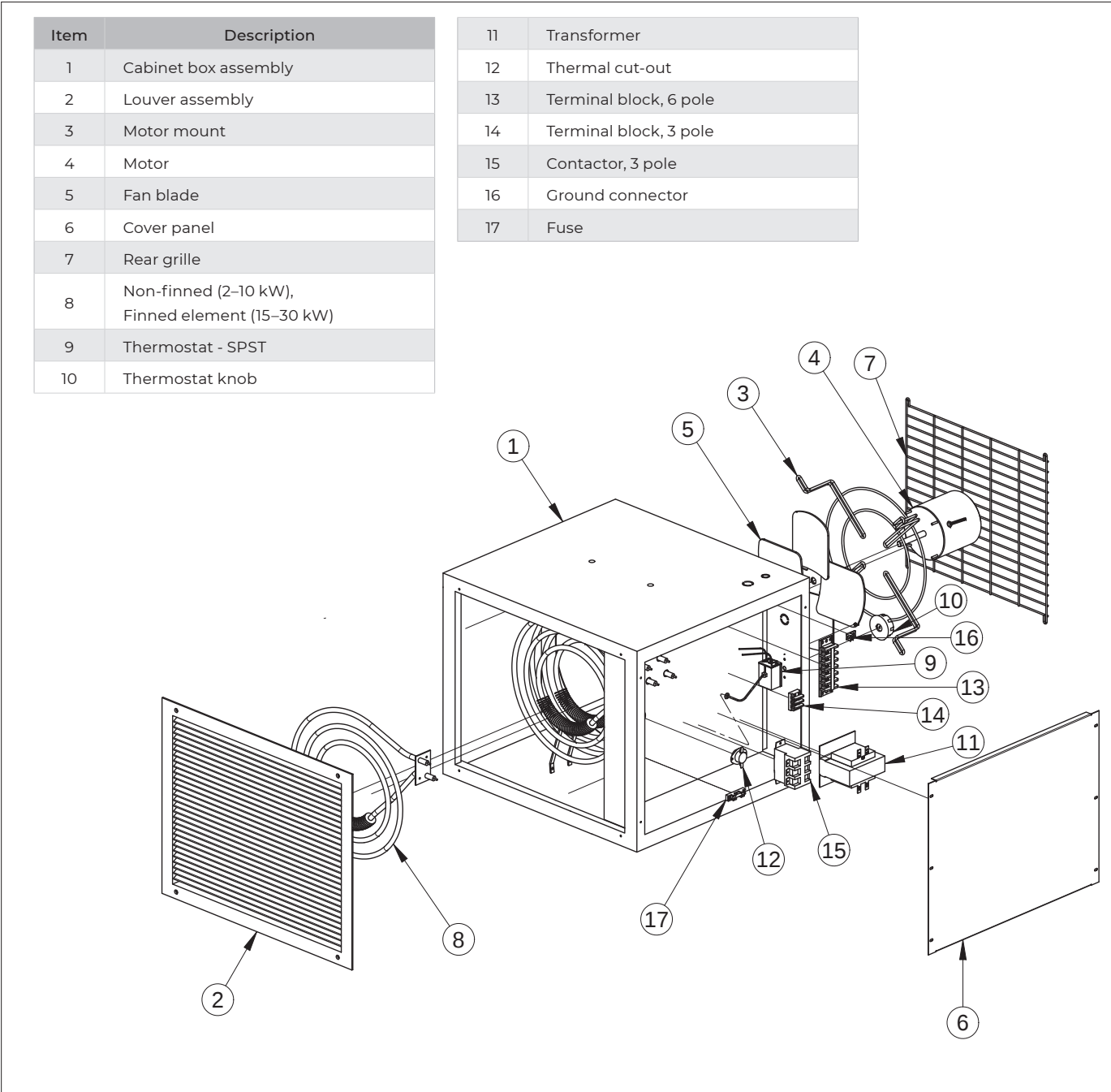
Figure 5 – Parts Assembly Diagram & Chart
