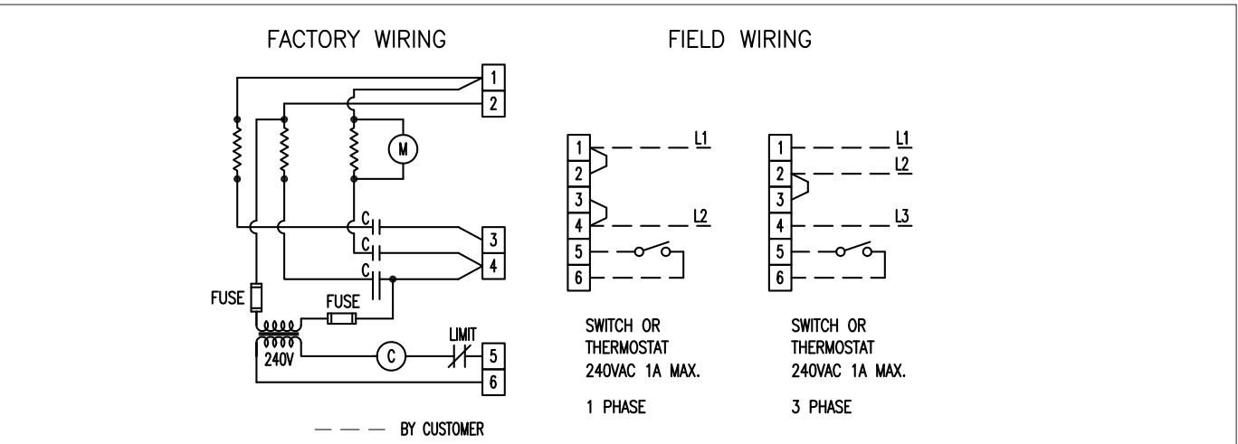
Figure 3G - GE Series 15–30 kW wiring schematic with hi-limit, contactor, transformer and fused control circuit options. 208–600V models.
