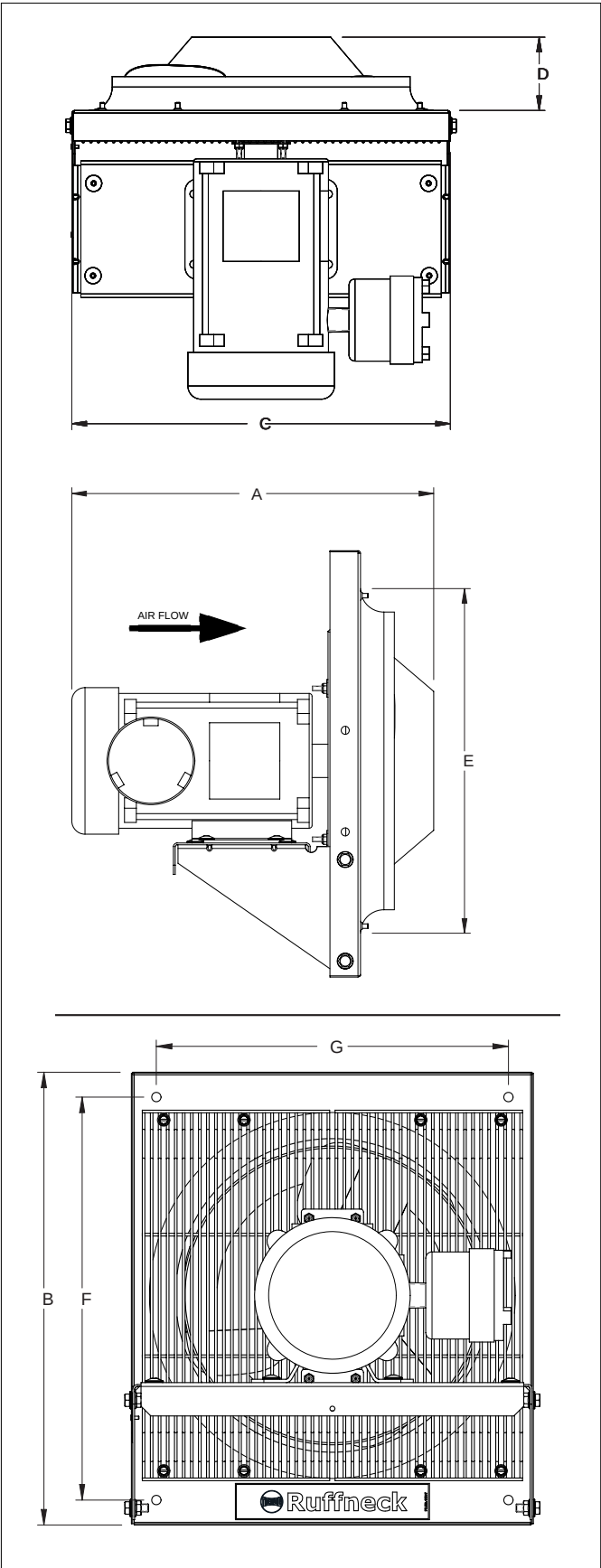
Figure 1 – Dimensions
