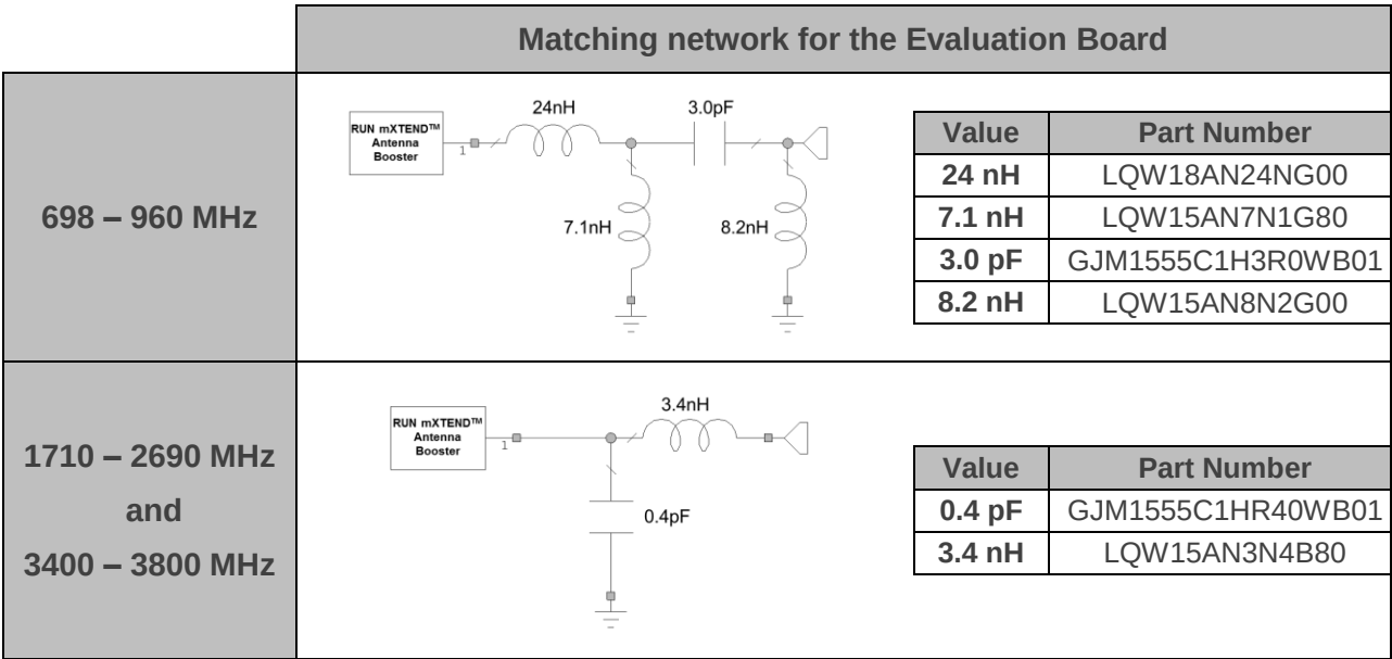
Figure 2 – Matching networks implemented in the Evaluation Board 2 ports (Figure 1).
