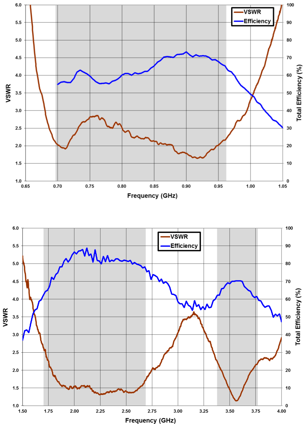
Figure 3 – VSWR and Total Efficiency for the 698 – 960 MHz range, for the 1710 – 2690 MHz, and for the 3400 – 3800 MHz range from the Evaluation Board 2 ports (Figure 1).
