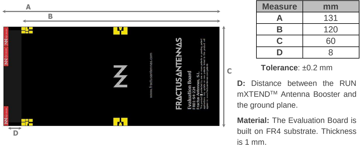
Figure 1 – EB_FR01-S4-224-UFL3R-2P. Evaluation Board providing operation in 3 frequency ranges, 698 MHz to 960 MHz, 1710 MHz to 2690MHz, and 3400 MHz to 3800 MHz.
