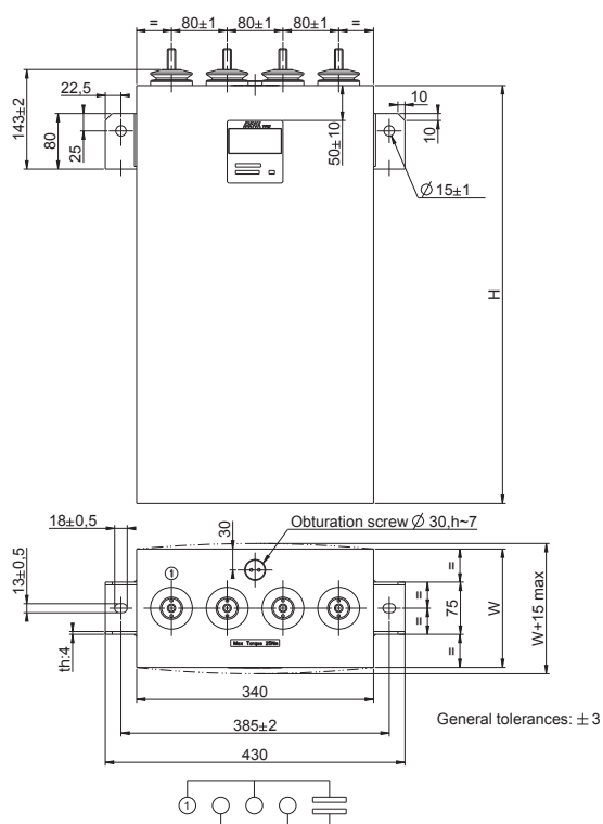
MALE TERMINALS
