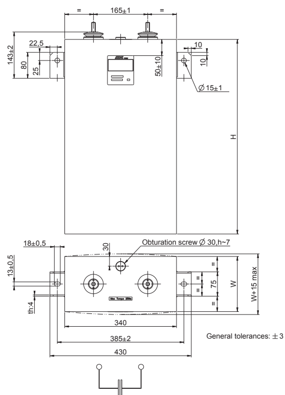
2 MALE TERMINALS
