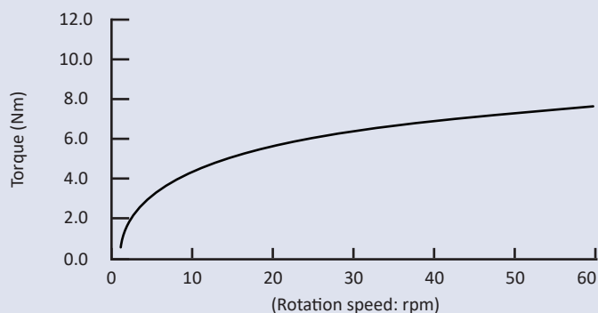
Speed characteristics of FDT-63A-533 series (Measurement temperature: 23°C)
