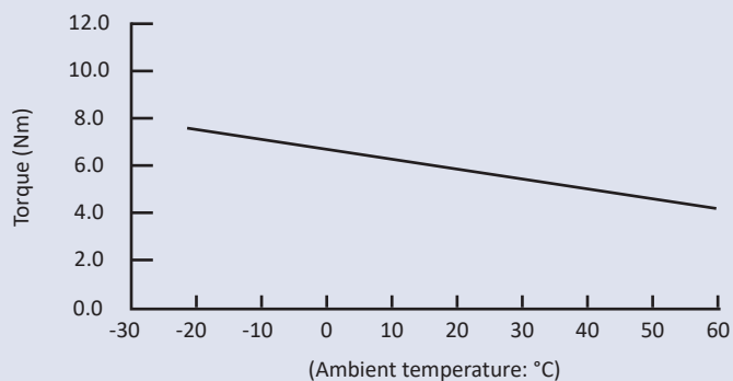
Temperature characteristics of FDT-63A-533 series (Rotation speed: 20 rpm)
