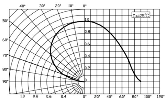
Radiation Diagram
