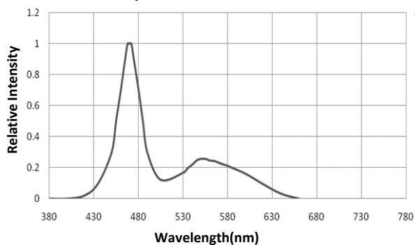
Spectrum Distribution
