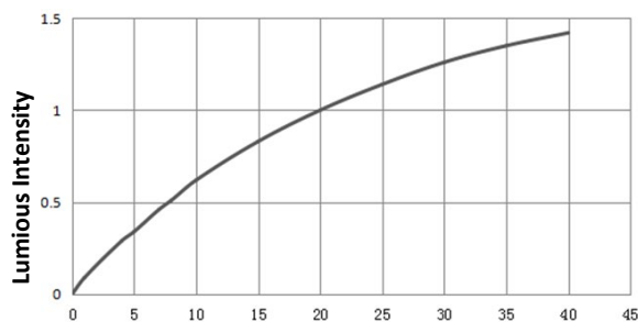
Luminous Intensity vs. Forward Current
