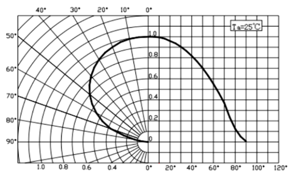
Radiation Diagram
