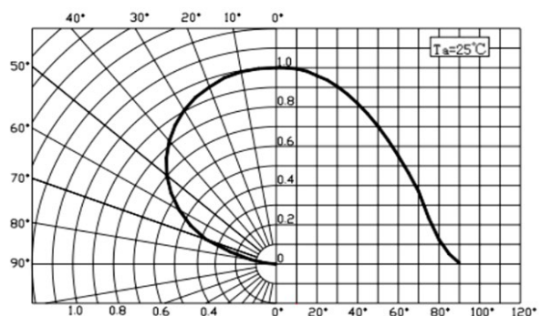
Radiation Diagram
