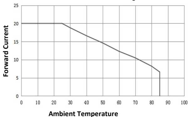
Forward Current Derating
