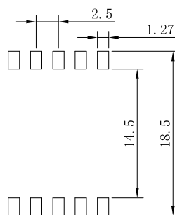
Recommended PAD Layout
