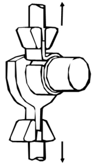
Figure 2. Part Specimen in Tensile Tester – (Rolling Drum Method Illustrated)
