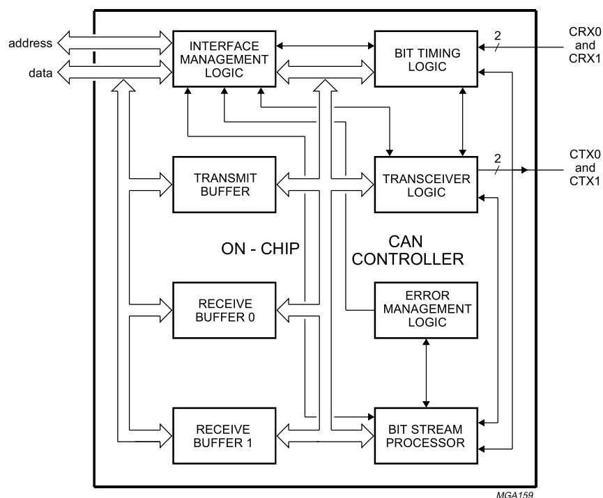
Fig.14 Block diagram of the P8xCE598 on-chip CAN-controller.
