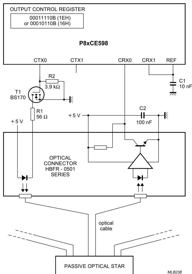
Fig.41 Optical Transceiver.
