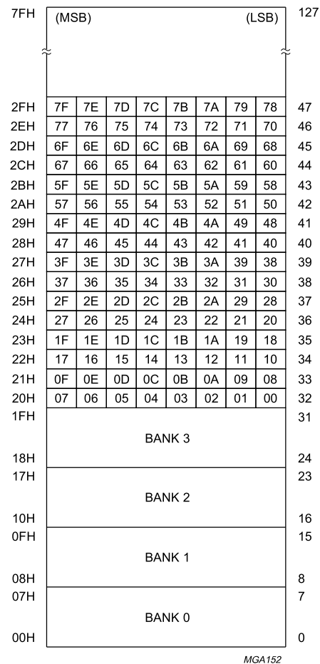
Fig.5 Internal MAIN RAM bit addresses.
