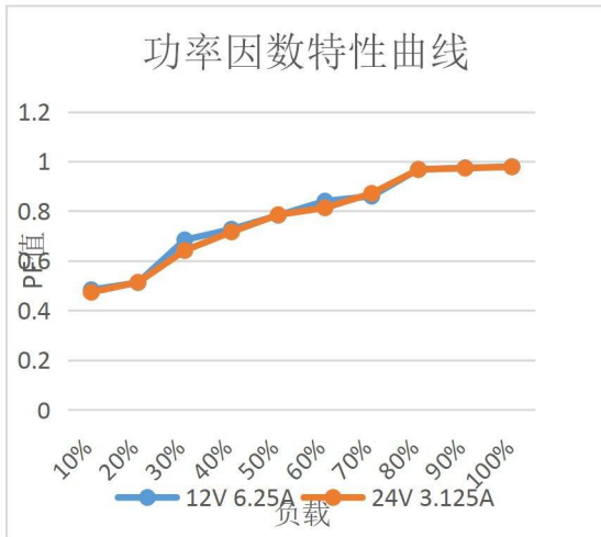
Power factor characteristic curve
