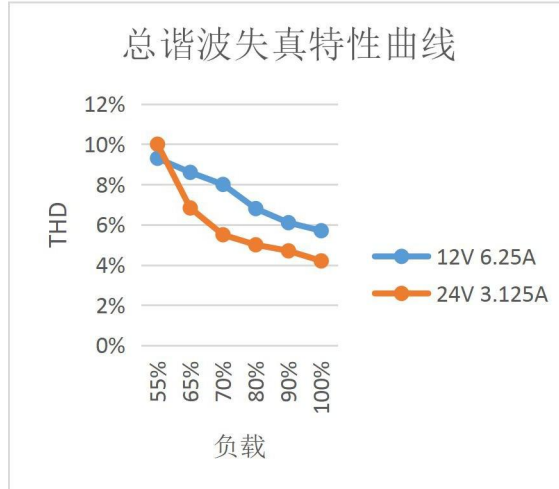
Total harmonic distortion characteristic curve
