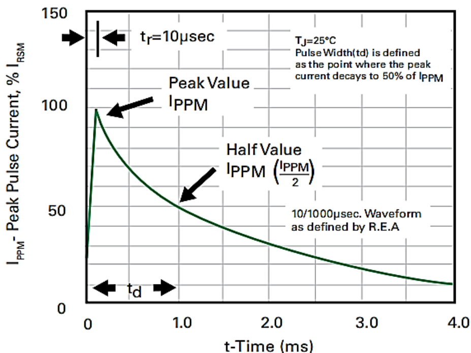
Figure 3. Pulse Waveform
