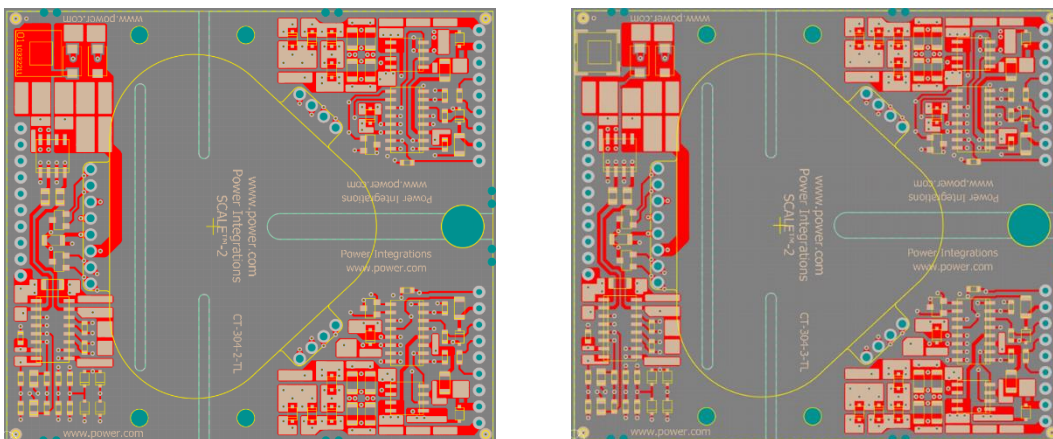
Fig. 2 Top Side 2SC0635T copper pour change in top left corner of PCB (left: old; right: new)
