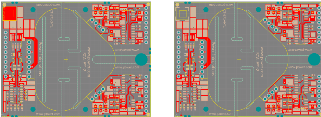
Fig. 1 Top Side 2SC0535T copper pour change in top left corner of PCB (left: old; right: new)
