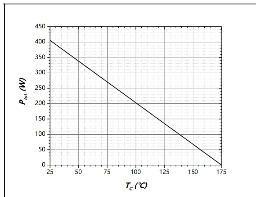
Figure 4. Power Derating
