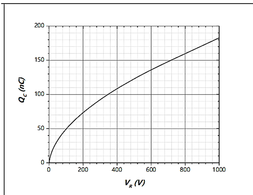
Figure 6. Total Capacitance Charge vs. Reverse Voltage
