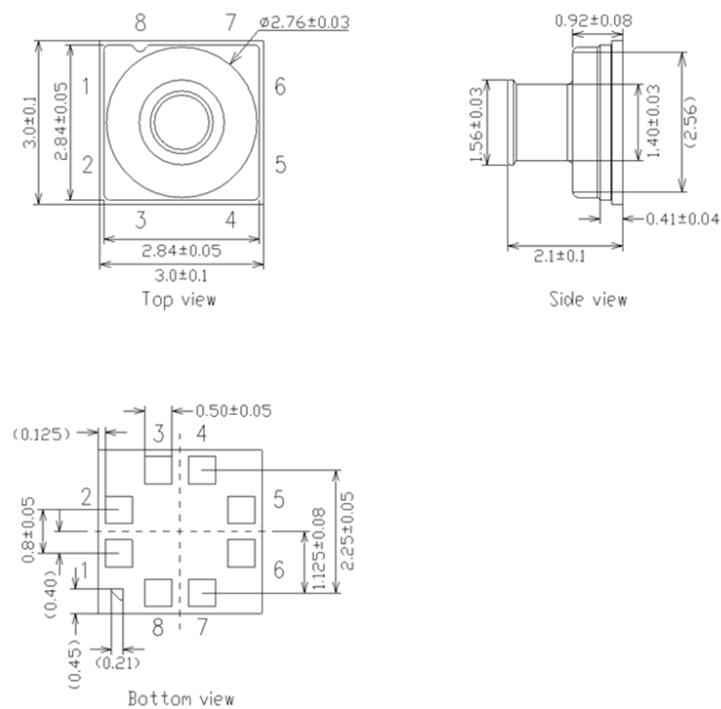
Figure 5. Package outline
