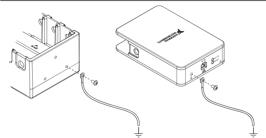
Figure 1-4. Ring Lug Attached to Ground Terminal
