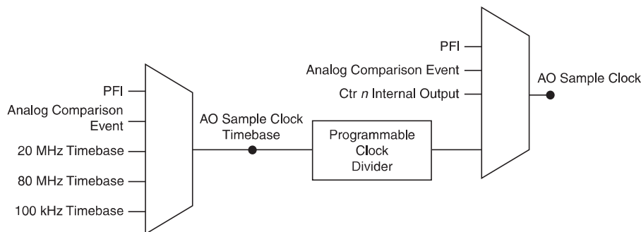
Figure 3-1. Analog Output Timing Options
