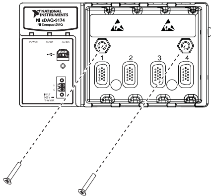
Figure 1-7. Mounting the cDAQ Chassis Directly on a Flat Surface
