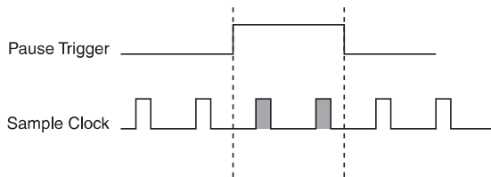
Figure 3-3. AO Pause Trigger with Other Signal Source
