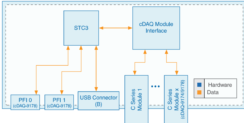
Figure 1-10. Block Diagram
