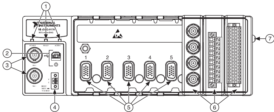
Figure 1-3. cDAQ-9178 Chassis
