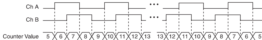
Figure 5-19. X4 Encoding
