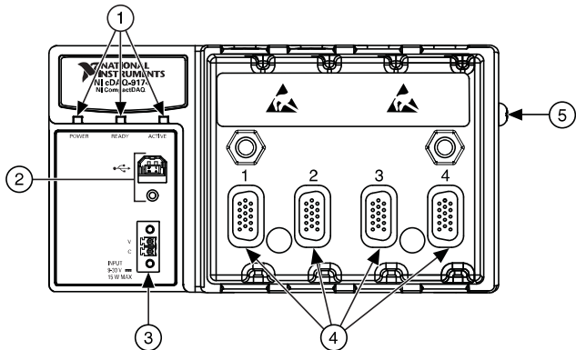
Figure 1-2. cDAQ-9174 Chassis
