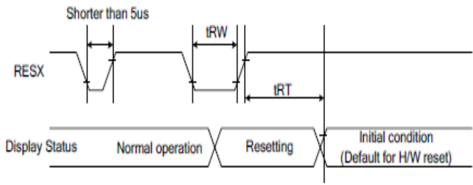
Figure 126: Reset Timing
