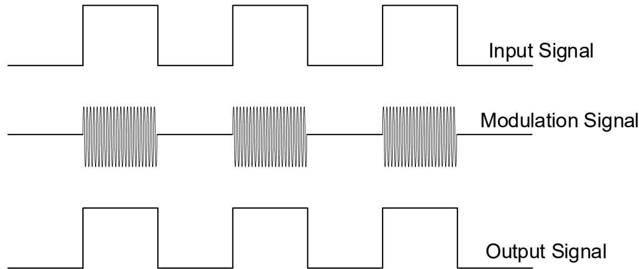
Figure 8. Modulation Scheme
