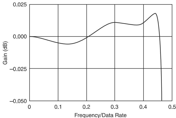
Figure 4. Typical Passband Flatness for the NI 9237
