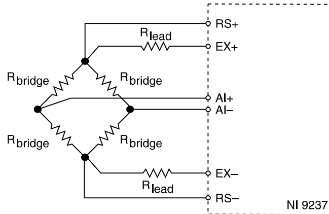
Figure 2. Connecting Remote Sense Wires to the NI 9237
