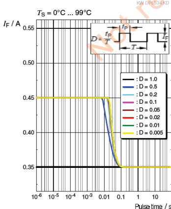
Permissible Pulse Handling Capability
