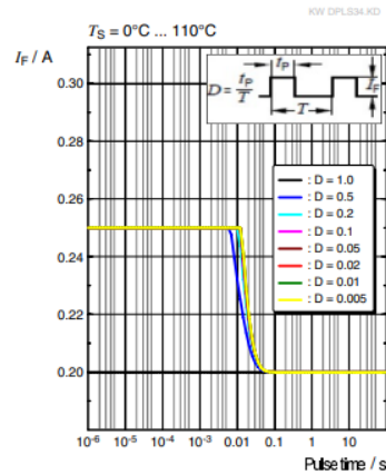
Permissible Pulse Handling Capability 7) I_F = f(t_p) ; D: Duty cycle
