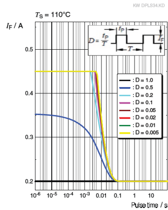
Permissible Pulse Handling Capability
