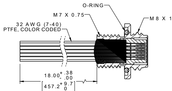
SECTION A-A LESS NUT
