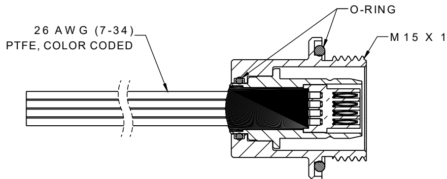
SECTION A-A LESS NUT
