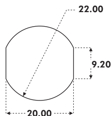
MOUNTING CUT-OUT
