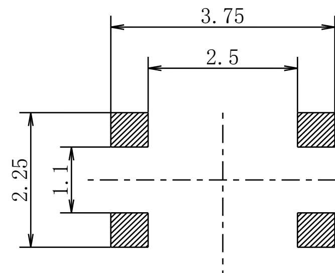
P. C. B LAND DIMENSION
