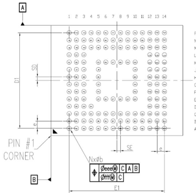
Figure 3 – Ball Pattern Dimensions
