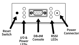
XTEND-PKG-R - FRONT
