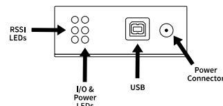
XTEND-PKG-U - FRONT
