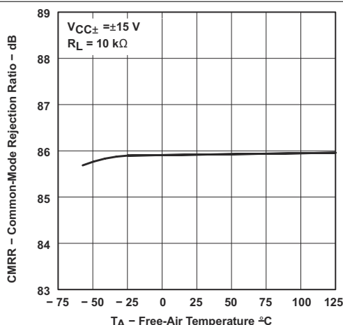
Figure 6-55. Common-Mode Rejection Ratio vs Free-Air Temperature
