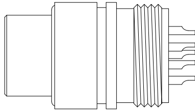
1x => CONNECTOR ENSURE O-RING IS ASSEMBLED ONTO CONNECTOR
