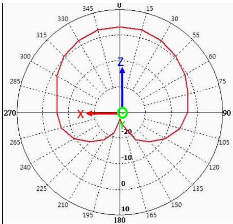
a) GNSS L1 Band @1575.42MHz (unit: dBi)
