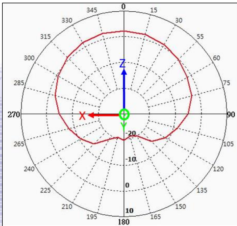
b) GNSS L5 Band @1176.5MHz (unit: dBi)
