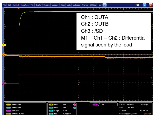
Figure 29. Zero pop noise turn on sequence with differential input to ground ( C_i = 100 \text{ nF} , R_i = 24 \text{ k}\Omega , R_f = 24 \text{ k}\Omega , C_{byp} = 1 \text{ }\mu\text{F} , R_l = 8 \text{ }\Omega , T_{on} = \text{GND} )
