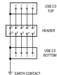
SCHEMATIC
