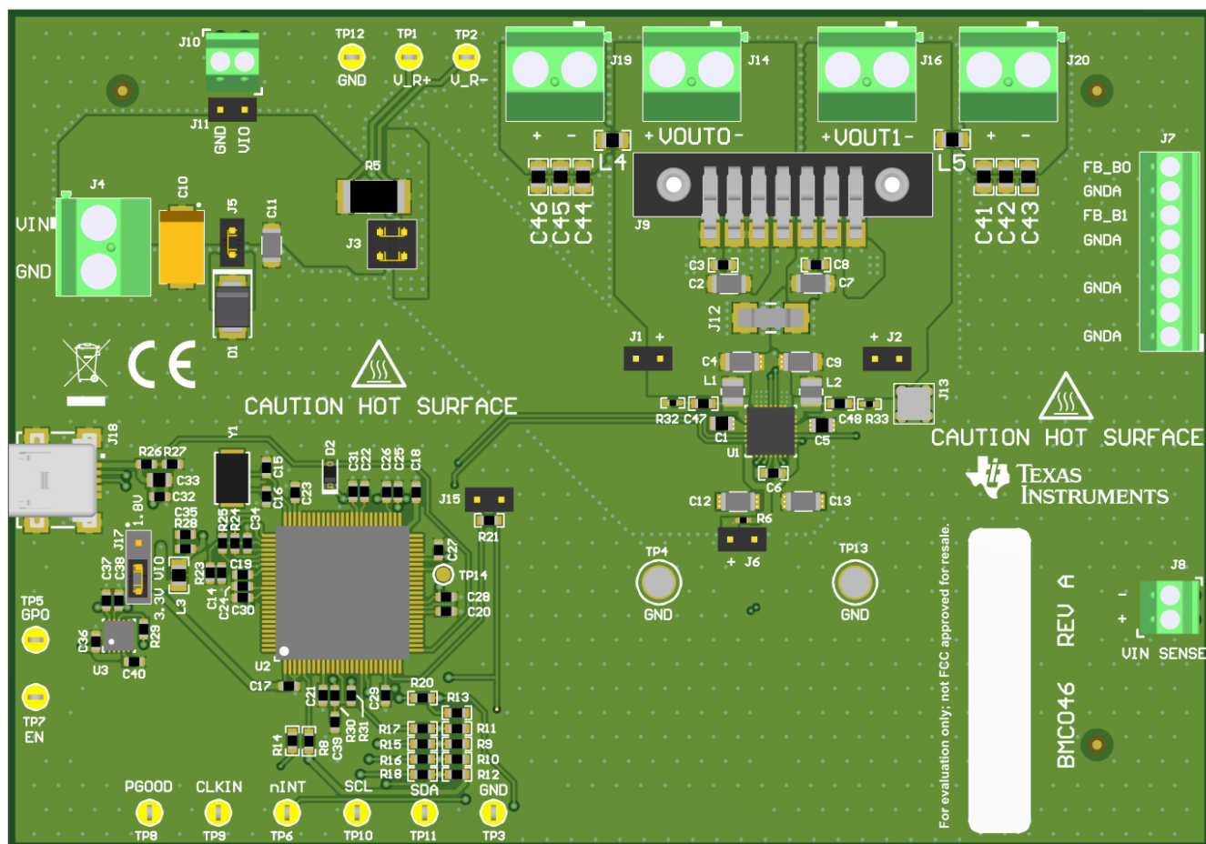
Figure 1. TPS65653-Q1 EVM
