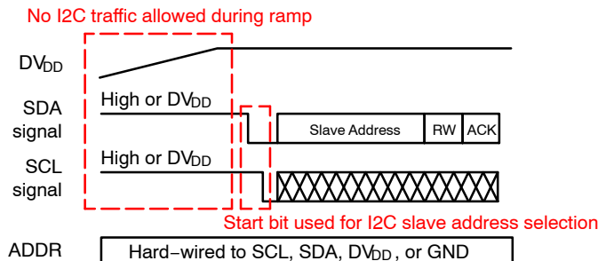
Figure 29. I 2 C Slave Address Selection on Power-up (ONA10IV)
