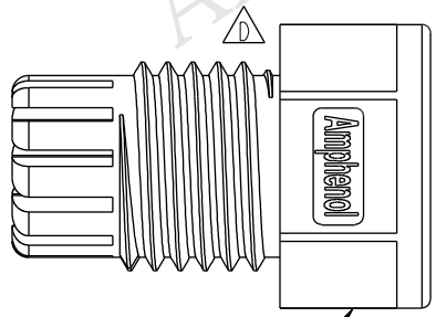
Clamp Ring (3)
