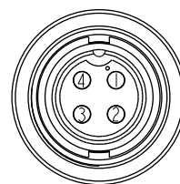
Pin Assignments Front View 前視圖
