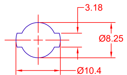
MOUNTING HOLE DIAGRAM MAXIMUM PANEL THICKNESS 1.19mm (.047")
