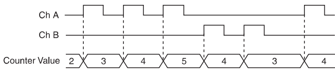
Figure 5-21. Measurements Using Two Pulse Encoders
