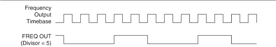
Figure 5-35. Frequency Generator Output Waveform
