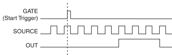
Figure 5-27. Single Pulse Generation with Start Trigger
