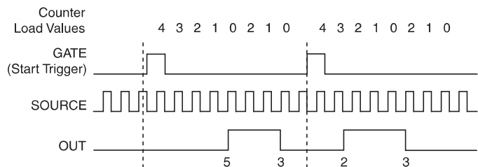
Figure 5-30. Retriggerable Single Pulse Generation False
