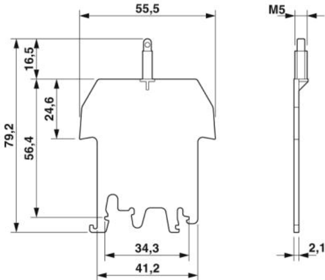
Dimensional drawing
