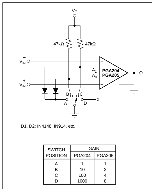
FIGURE 6. Switch-Selected PGIA.
