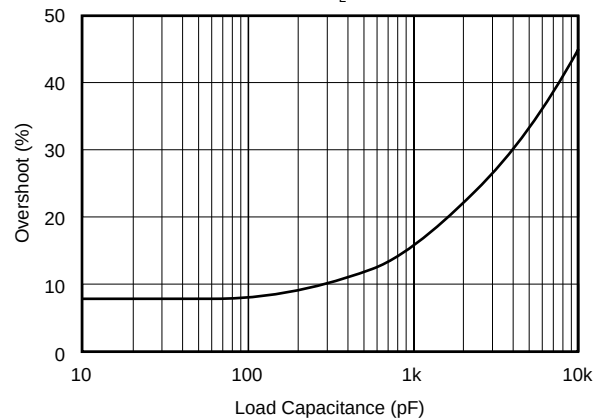
OVERSHOOT vs LOAD CAPACITANCE ( G = +1 , R_L = 1k\Omega )
