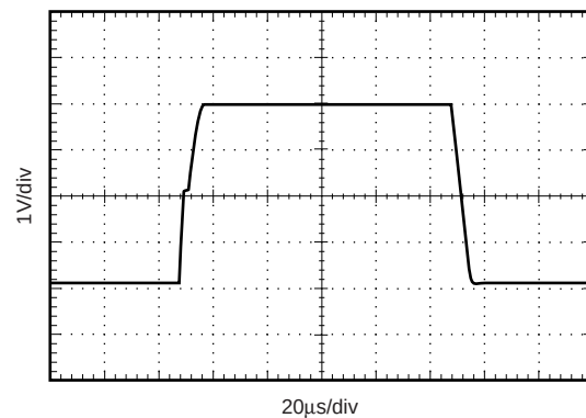
LARGE-SIGNAL STEP RESPONSE ( G = +1 , R_L = 1\Omega )
