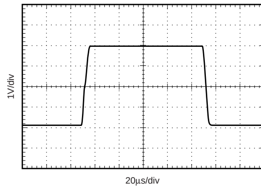
LARGE-SIGNAL STEP RESPONSE ( G = +1 , R_L = 10\Omega )
