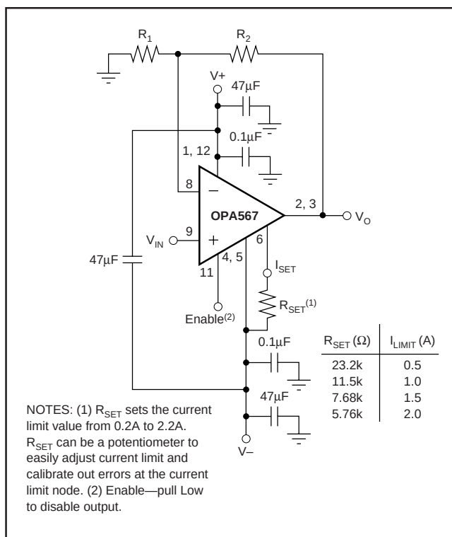
FIGURE 1. Basic Connections.
