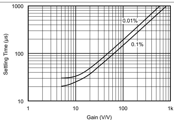
Figure 8. Settling Time vs Gain
