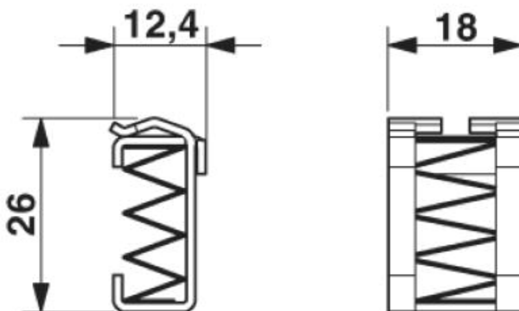
Dimensional drawing
