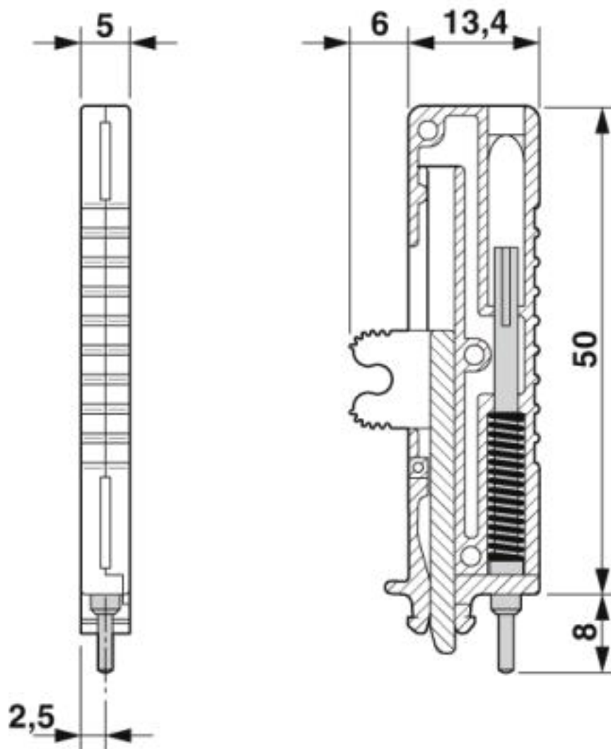
Dimensional drawing
