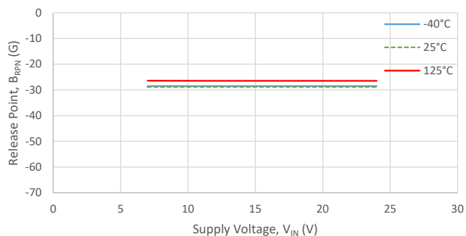
Release Point, North ( B_{RPN} v. V_{IN} )
